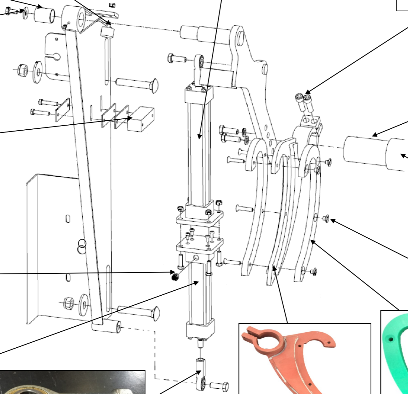
34879400 Pneumatic Cylinder x 2
